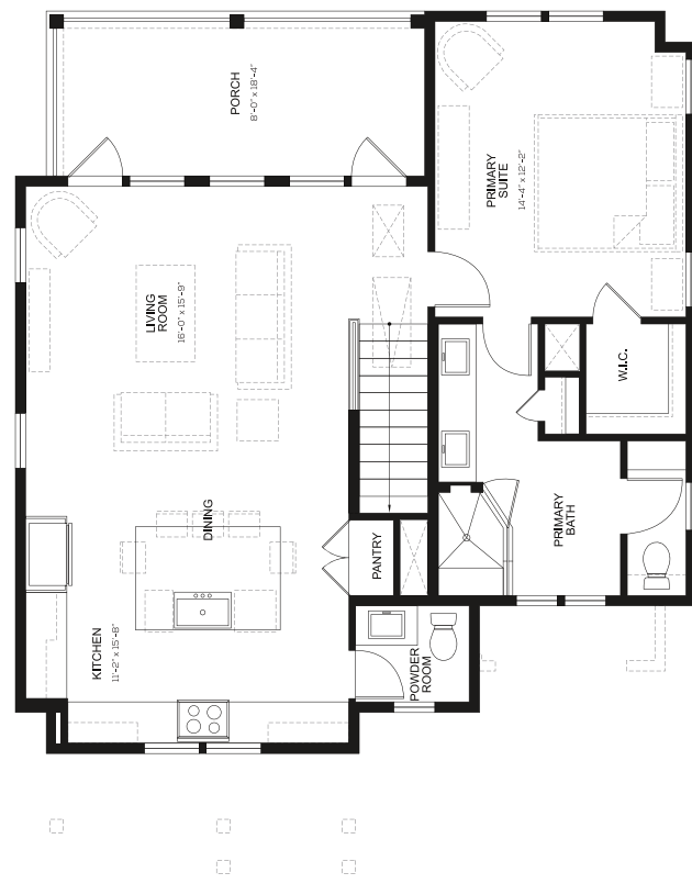
SECOND FLOOR
